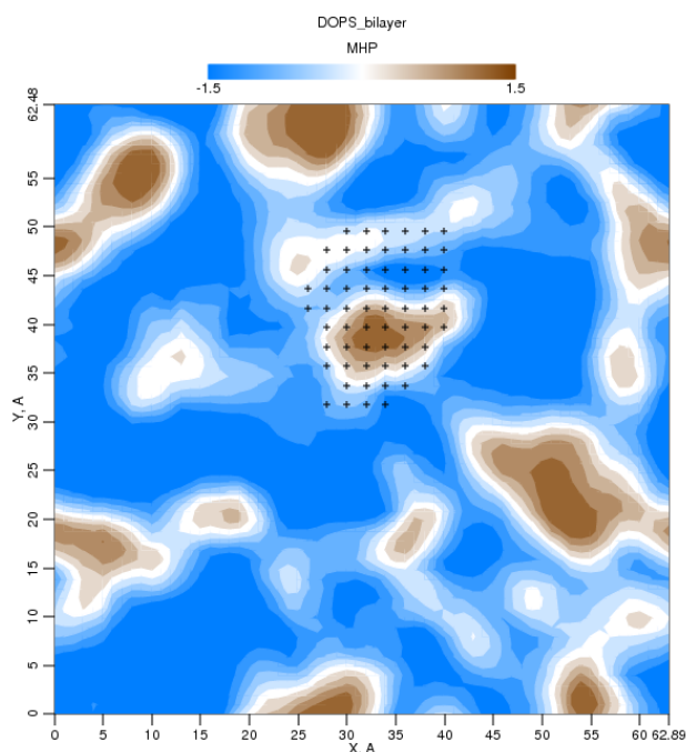
Figure 2.4. An example of 2D-hydrophobicity map of a dioleoylphosphatidylserine (DOPS) layer. A membrane-active peptide approaching the membrane (uploaded as ligand) is projected onto the map in “shadow” mode (depicted with crosses).
