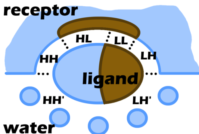
Figure 1.3. Types of contacts between ligand and its environment on ligand molecular surface. Each dot type corresponds to different combination of ligand and environmental MHP (i.e. hydrophobic/hydrophilic properties). Character “L” means lipophilic (brown, oil-colored) and “H” – hydrophilic (blue, water-colored). Apostrophe symbol designates exposed ligand surface which is in contact with hydrophilic solvent.
