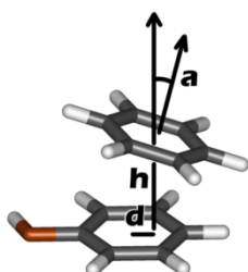
Figure 1.4. Scheme of geometrical parameters used to describe a stacking contact between two aromatic rings. Displacement ( d ) and height ( h ) are calculated for the center of one aromatic ring relative to another ring's plane. Angle \alpha is calculated as the angle between the normal vectors of both rings.
