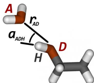
Figure 1.5. Scheme of geometrical parameters used to describe a hydrogen bond.
