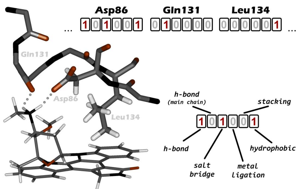
Figure 1.6. An example of IFP bit string. Inhibitor staurosporin is shown in Cyclin-Dependent Kinase 2 active site (PDB code 1AQ1). Interactions of selected residues are shown as they are encoded into an IFP bit string.
