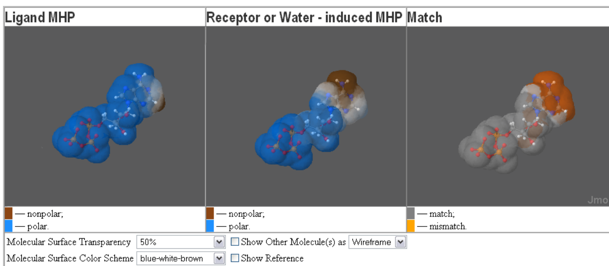
Figure 2.6. Visualization in online Jmol applet. User can choose surface transparency and MHP color scheme to display the ligand own (left panel) and its receptor (middle panel) hydrophobic/hydrophilic properties. The right panel maps match (grey) and mismatch (orange) of the properties of the ligand and its environment.
